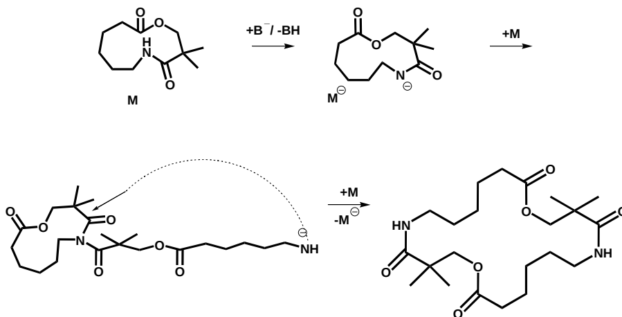
Figure 11. Polymerization mechanism of cyclic 11-membered ester amides.
