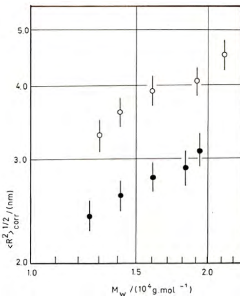
Figure 15. Radius of gyration as a function of molecular weight for cyclic (•) and acyclic (o) polystyrene as obtained from low angle neutron scattering in toluene- d_8 .
